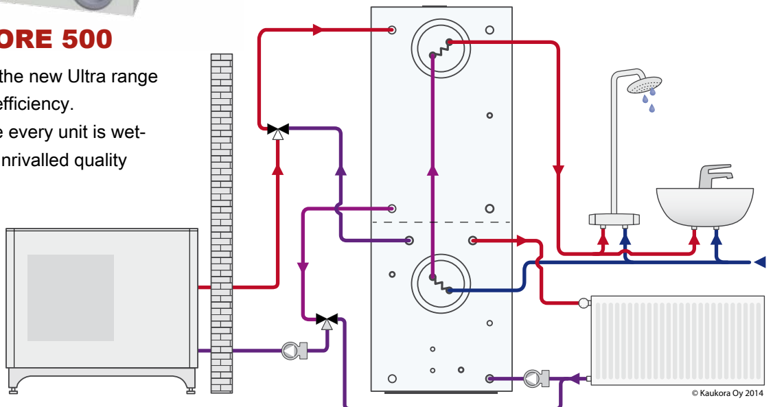
Ultrastore 500 with Heat Pump, Radiators and Domestic Hot Water
